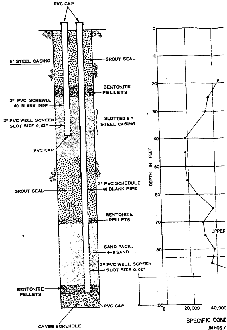
WELL COMPLETION LOG
