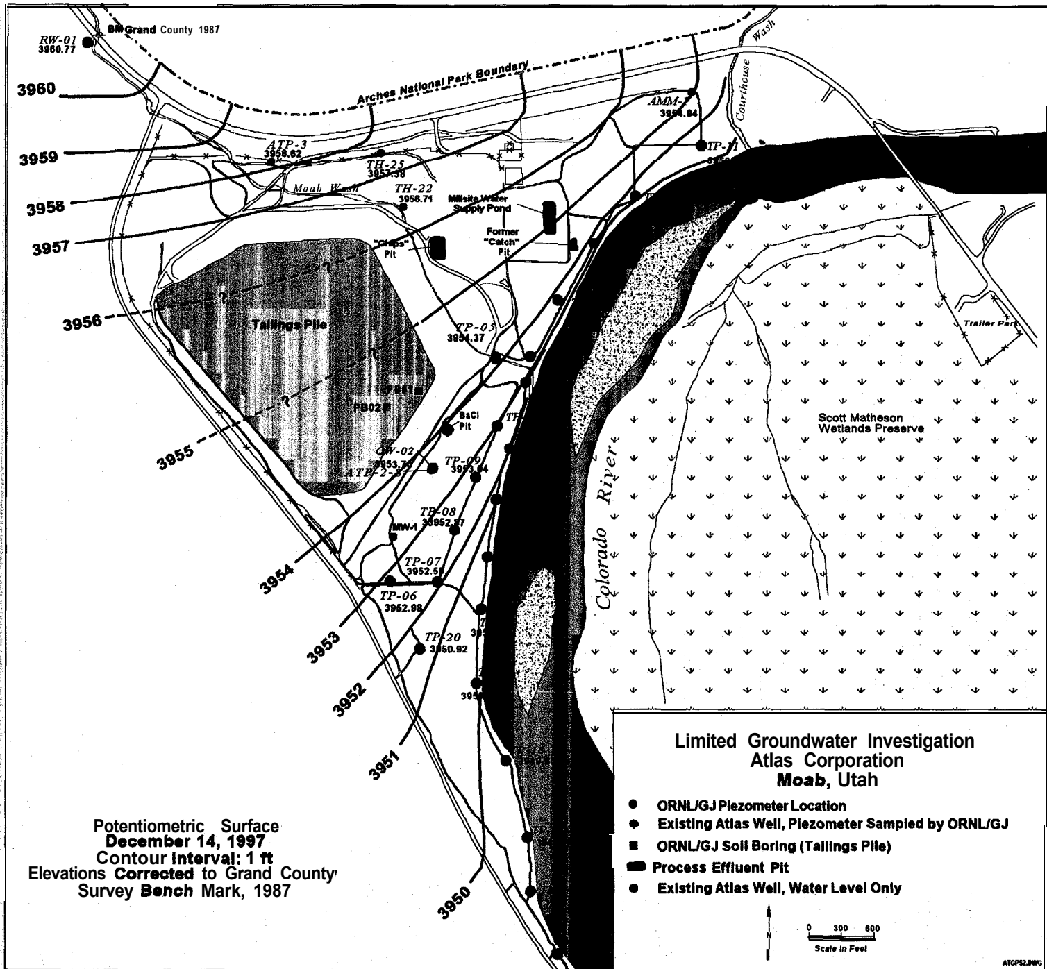
Fig. 3.6. Potentiometric surface map for shallow alluvial aquifer, December 14, 1997.
